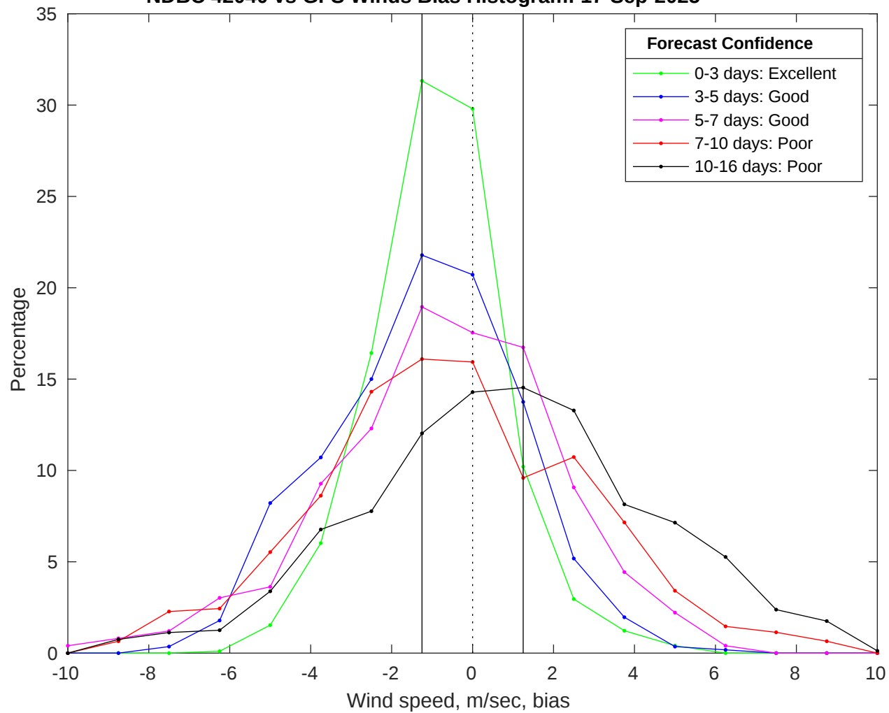
NDBC 42040 vs GFS Winds Bias Histogram: 17-Sep-2025
