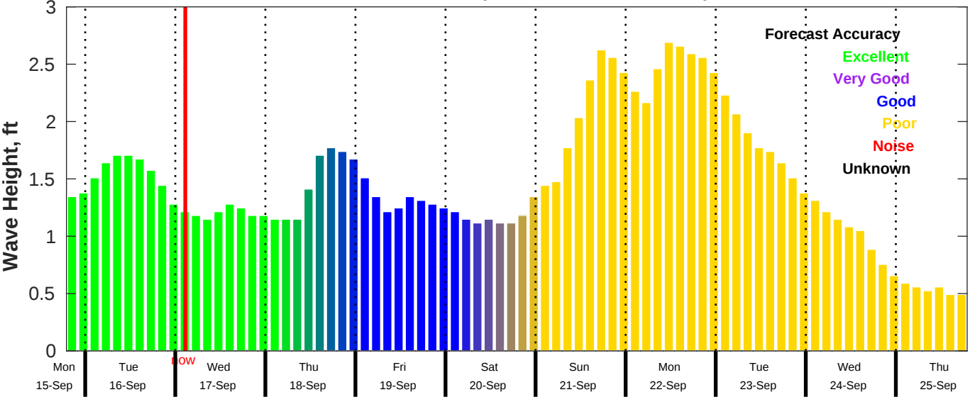
CMEMS Wave Forecast for NDBC 42040 from 15-Sep-2025 19:00:00 to 25-Sep-2025 19:00:00
