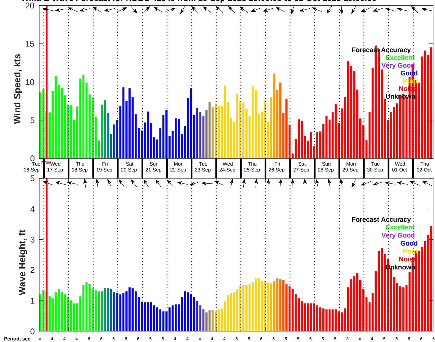
Wind & Wave Forecast for NDBC 42040 from 16-Sep-2025 19:00:00 to 02-Oct-2025 19:00:00
