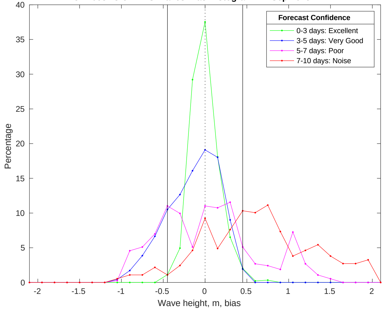
NDBC 44008 vs CMEMS Waves Bias Histogram: 17-Sep-2025
