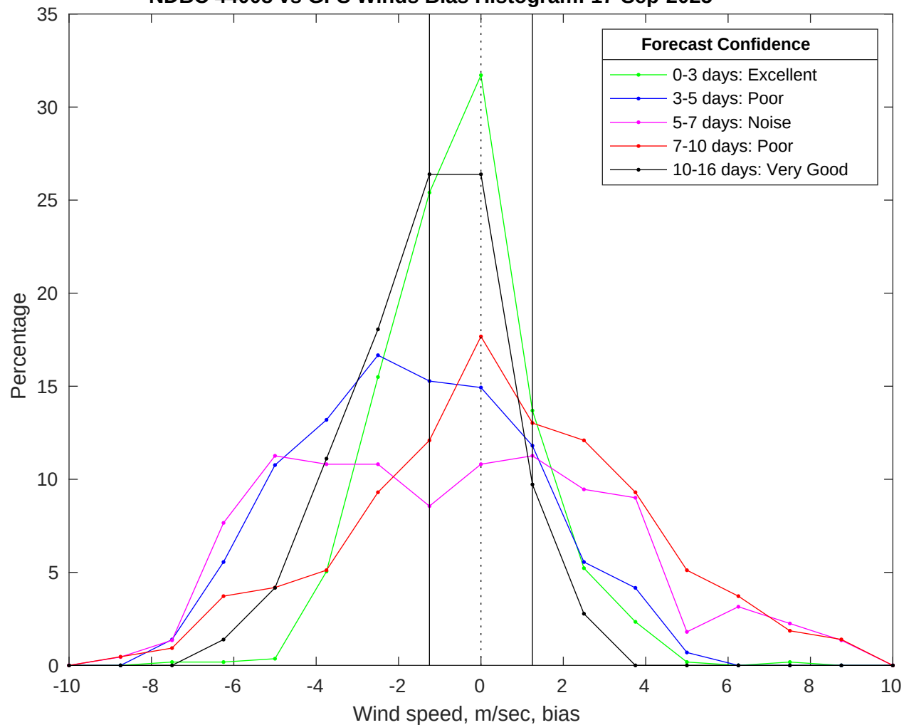
NDBC 44008 vs GFS Winds Bias Histogram: 17-Sep-2025
