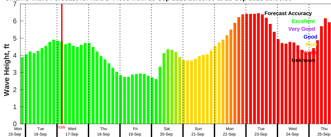
CMEMS Wave Forecast for NDBC 44008 from 15-Sep-2025 20:00:00 to 25-Sep-2025 20:00:00
