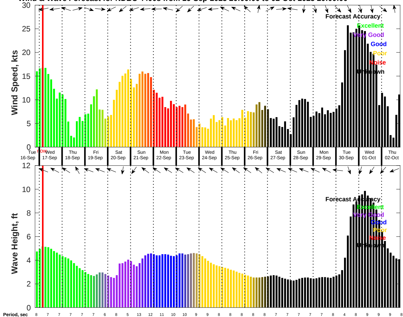
Wind & Wave Forecast for NDBC 44008 from 16-Sep-2025 20:00:00 to 02-Oct-2025 20:00:00
