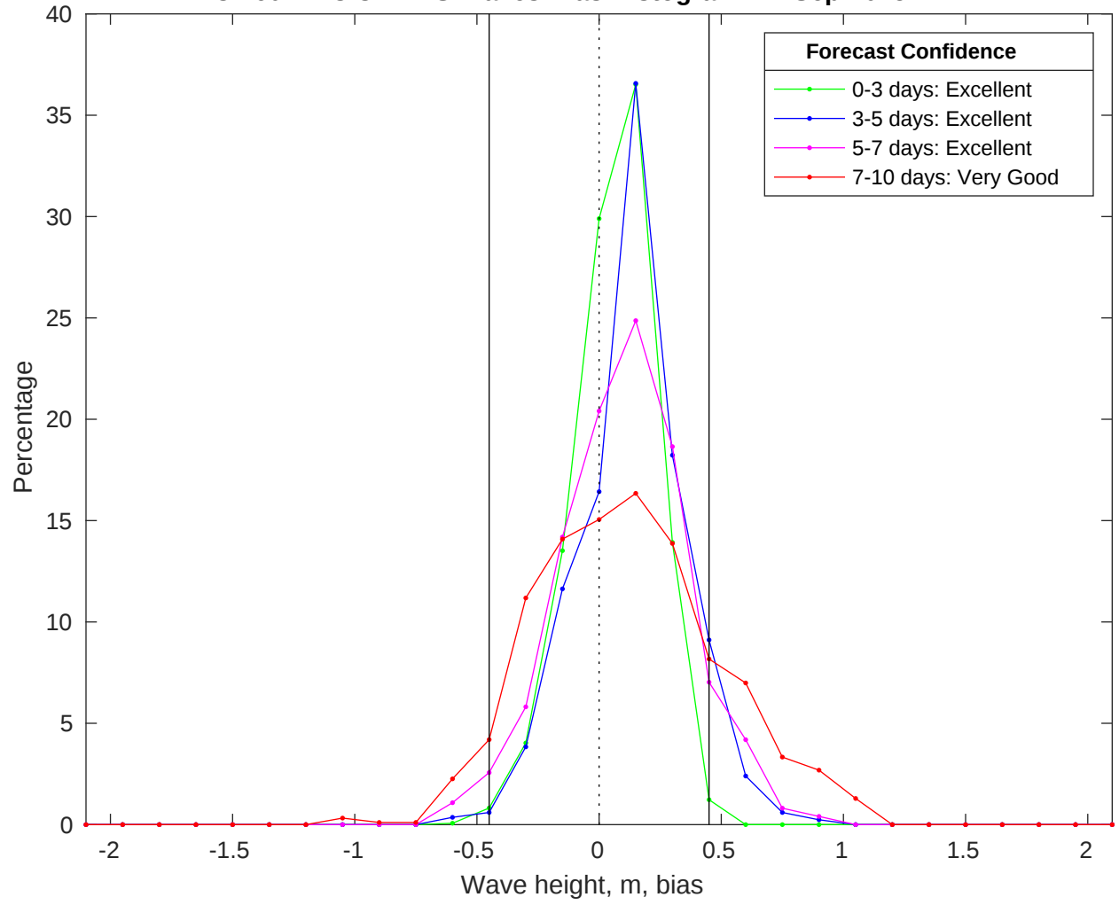
NDBC 46011 vs CMEMS Waves Bias Histogram: 17-Sep-2025
