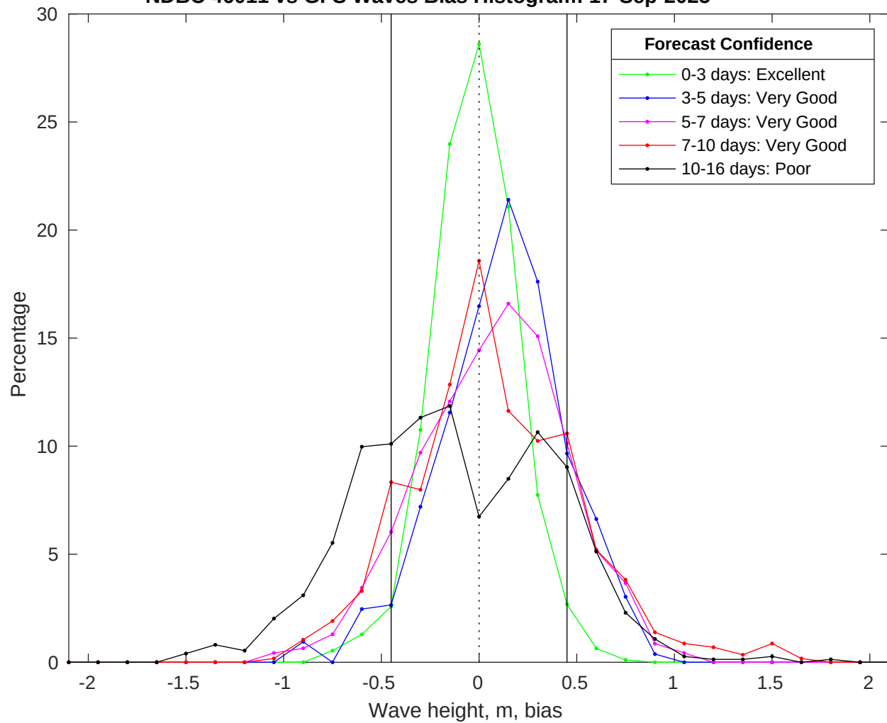
NDBC 46011 vs GFS Waves Bias Histogram: 17-Sep-2025
