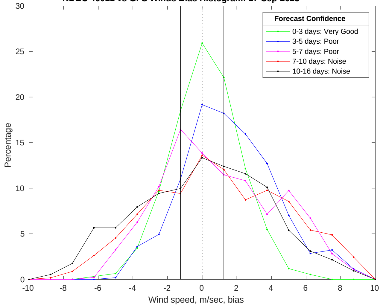
NDBC 46011 vs GFS Winds Bias Histogram: 17-Sep-2025
