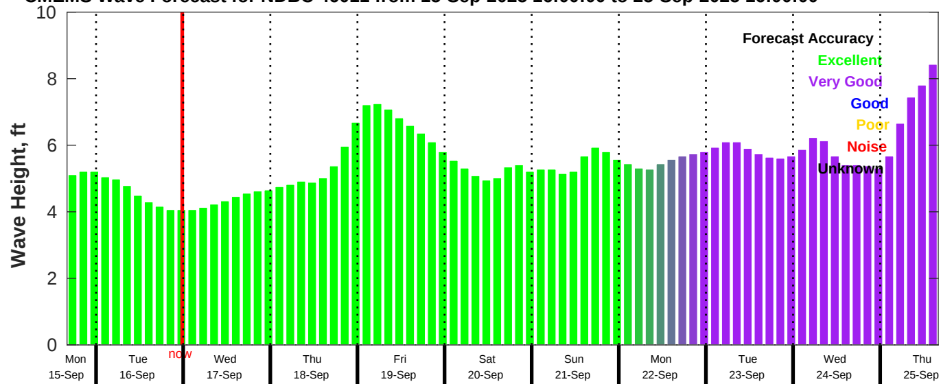
CMEMS Wave Forecast for NDBC 46011 from 15-Sep-2025 16:00:00 to 25-Sep-2025 16:00:00
