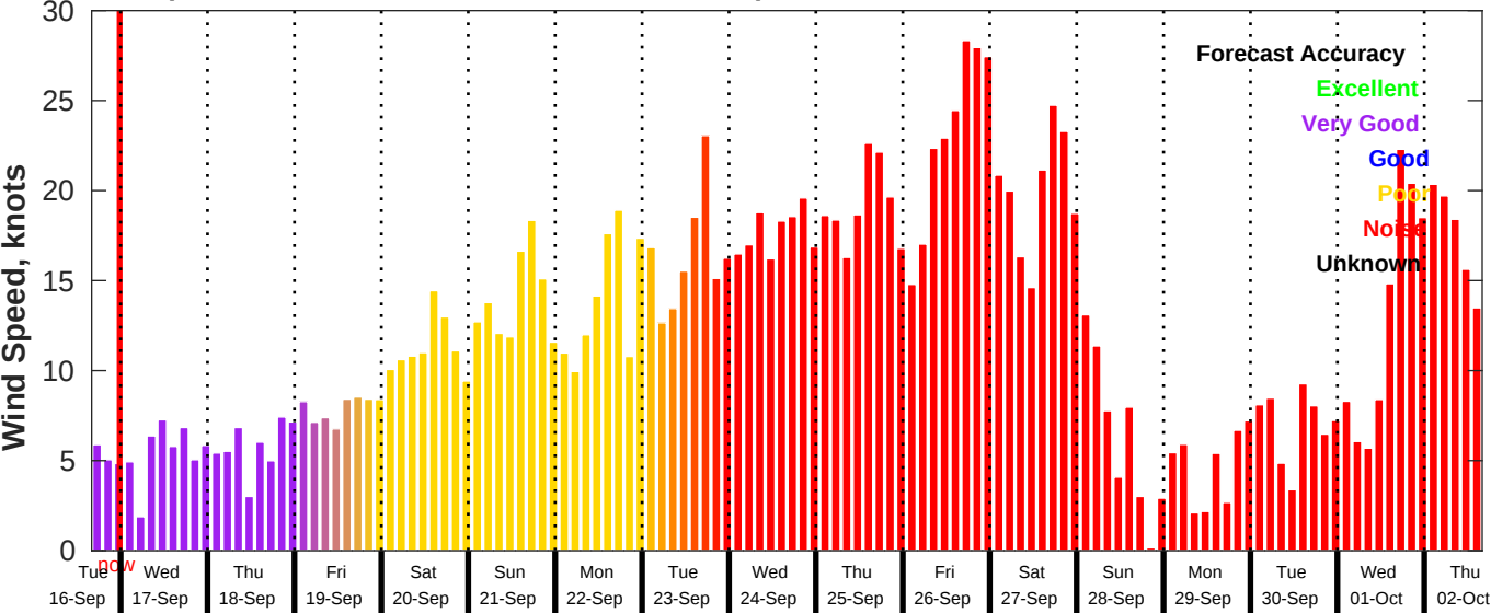
GFS Wind Speed Forecast for NDBC 46011 from 16-Sep-2025 16:00:00 to 02-Oct-2025 16:00:00
