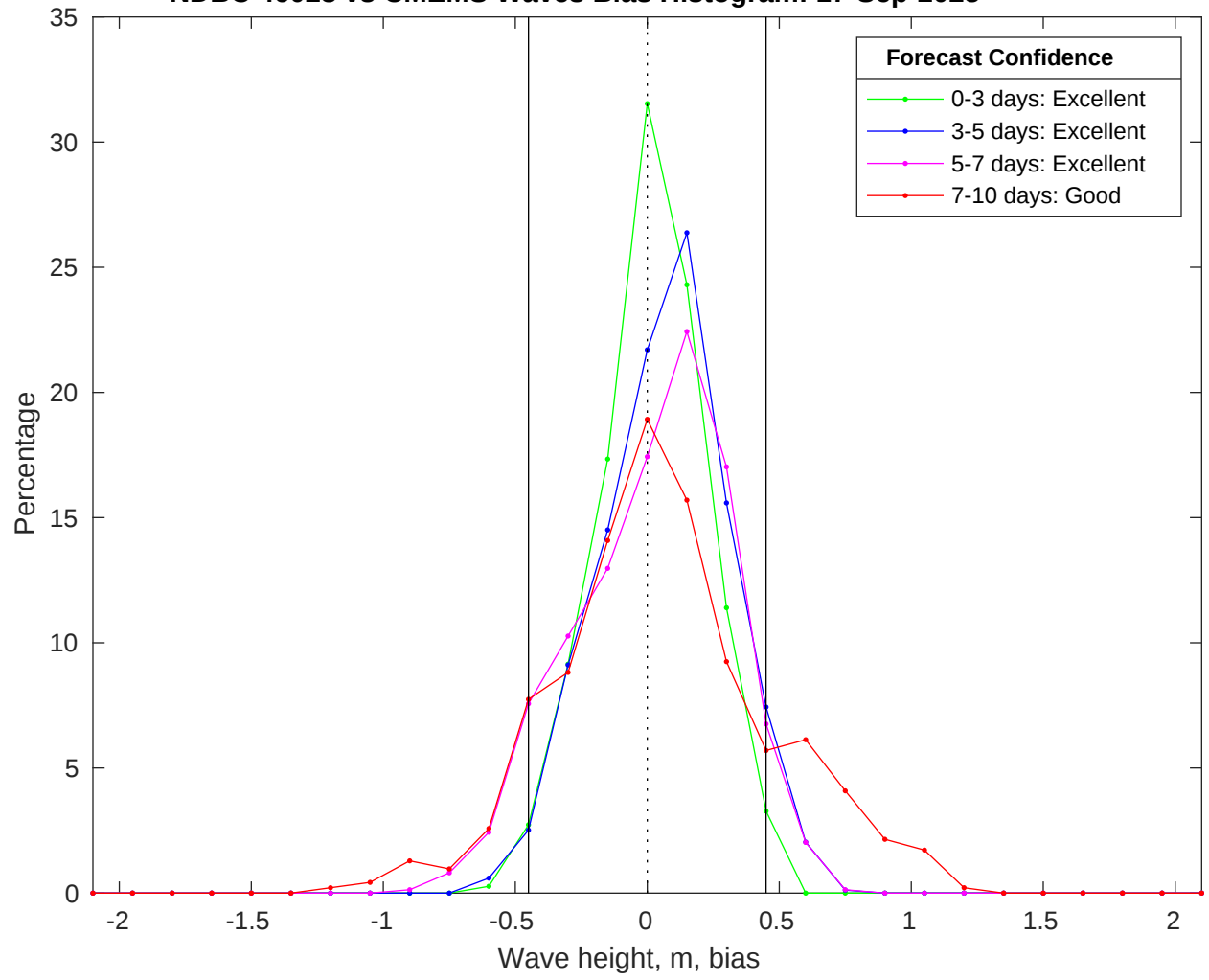
NDBC 46028 vs CMEMS Waves Bias Histogram: 17-Sep-2025
