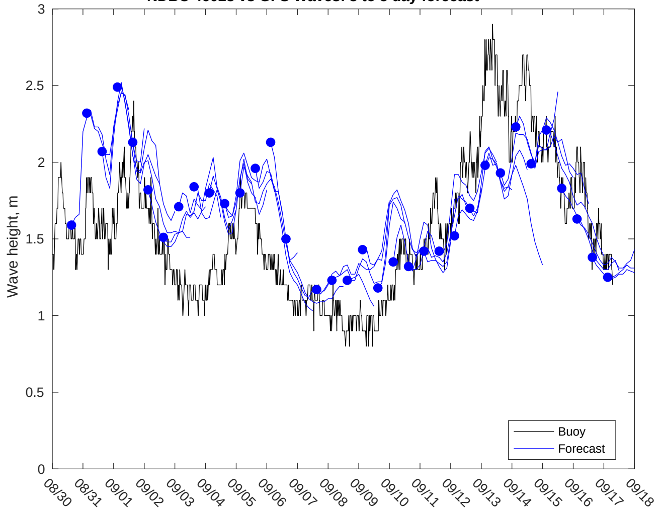
NDBC 46028 vs GFS Waves: 3 to 5 day forecast
