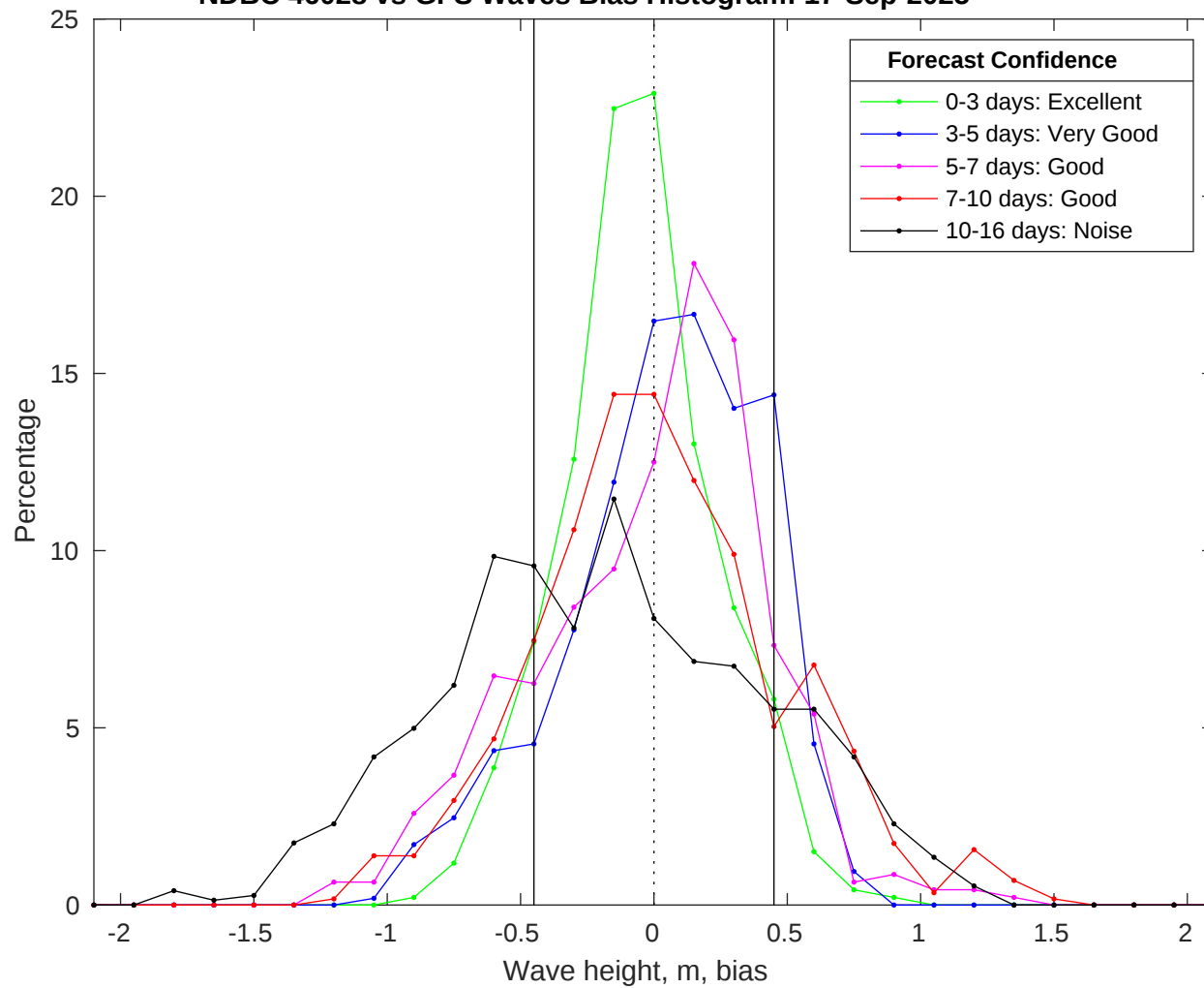
NDBC 46028 vs GFS Waves Bias Histogram: 17-Sep-2025
