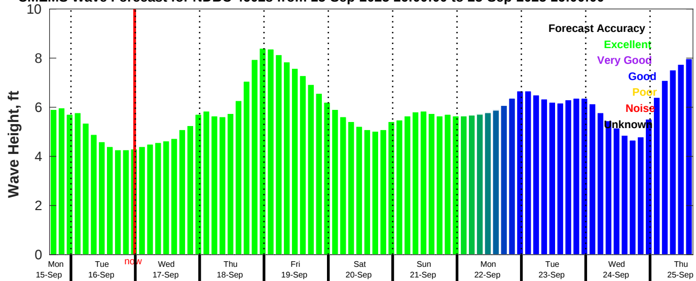
CMEMS Wave Forecast for NDBC 46028 from 15-Sep-2025 16:00:00 to 25-Sep-2025 16:00:00
