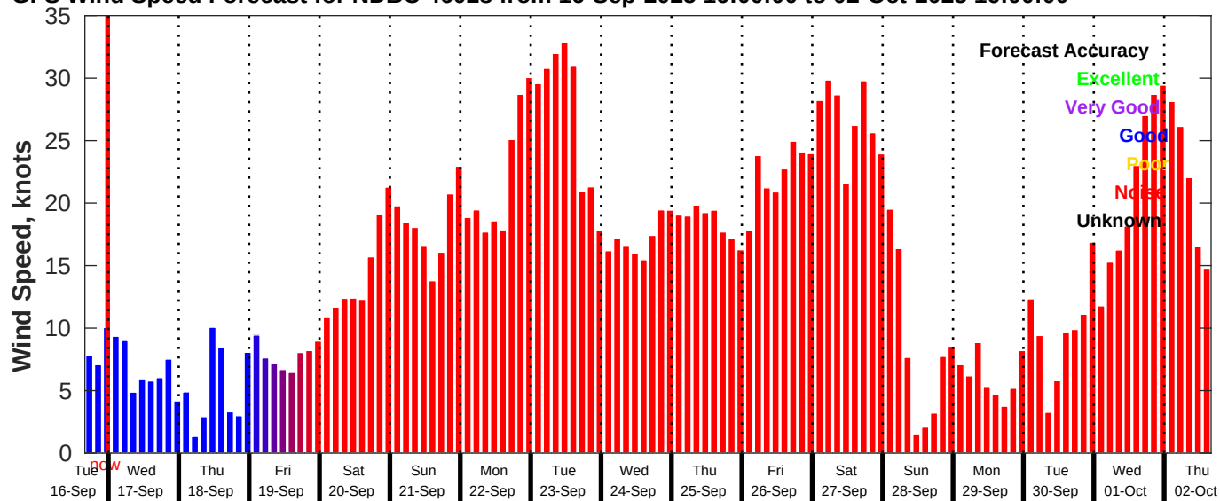
GFS Wind Speed Forecast for NDBC 46028 from 16-Sep-2025 16:00:00 to 02-Oct-2025 16:00:00
