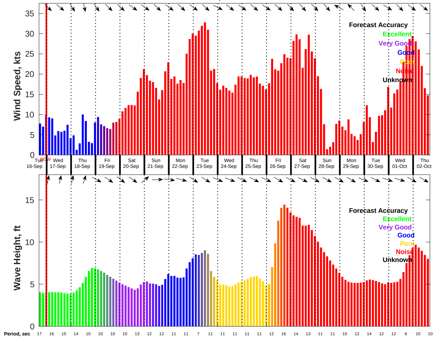
Wind & Wave Forecast for NDBC 46028 from 16-Sep-2025 16:00:00 to 02-Oct-2025 16:00:00
