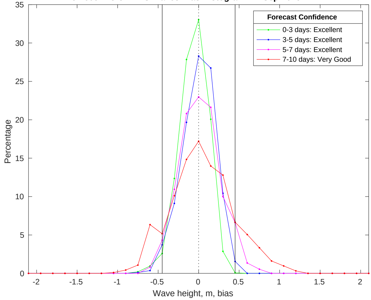
NDBC 46054 vs CMEMS Waves Bias Histogram: 17-Sep-2025
