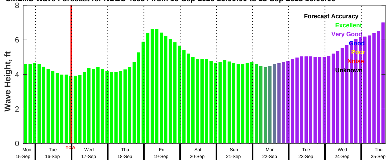
CMEMS Wave Forecast for NDBC 46054 from 15-Sep-2025 16:00:00 to 25-Sep-2025 16:00:00
