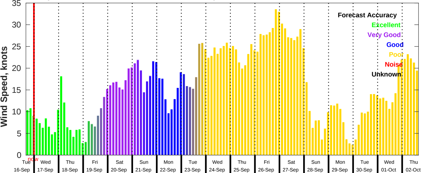
GFS Wind Speed Forecast for NDBC 46069 from 16-Sep-2025 16:00:00 to 02-Oct-2025 16:00:00
