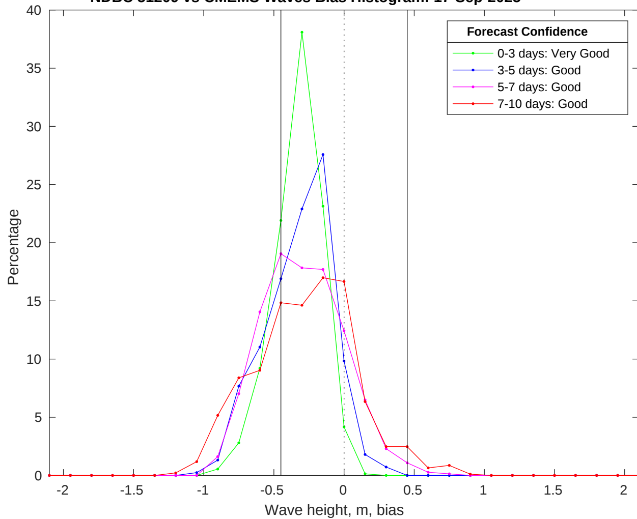
NDBC 51209 vs CMEMS Waves Bias Histogram: 17-Sep-2025
