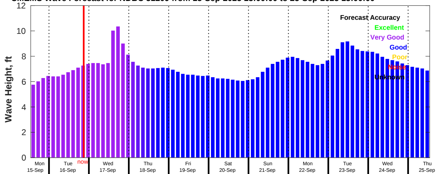
CMEMS Wave Forecast for NDBC 51209 from 15-Sep-2025 13:00:00 to 25-Sep-2025 13:00:00
