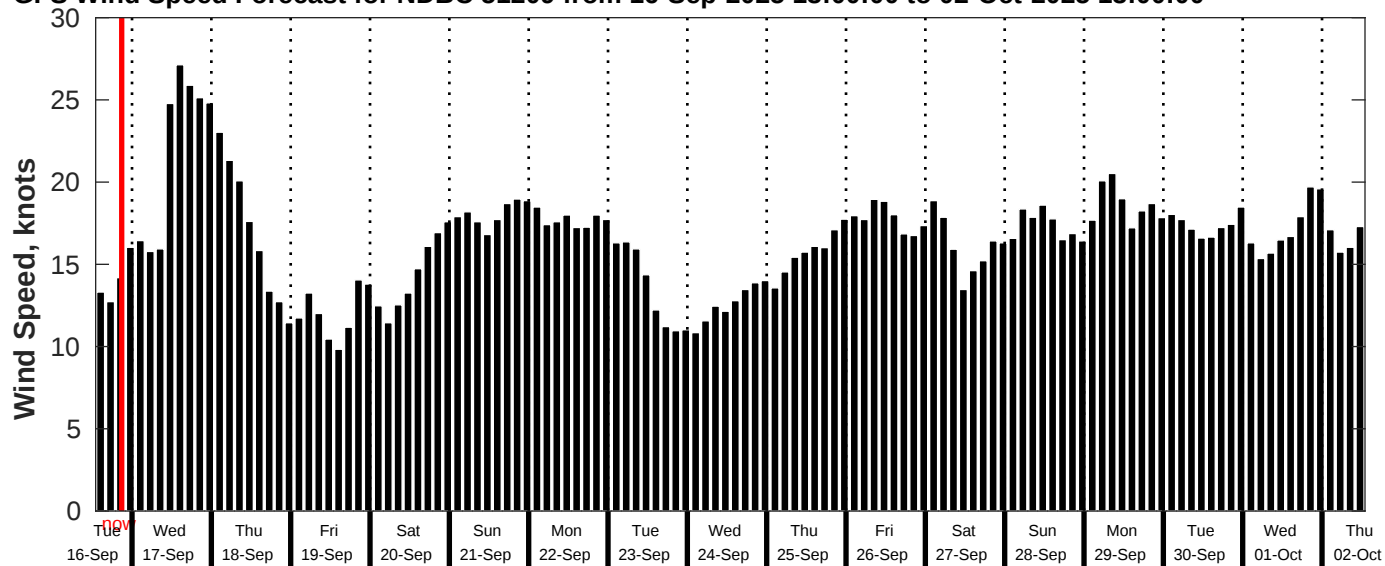
GFS Wind Speed Forecast for NDBC 51209 from 16-Sep-2025 13:00:00 to 02-Oct-2025 13:00:00
