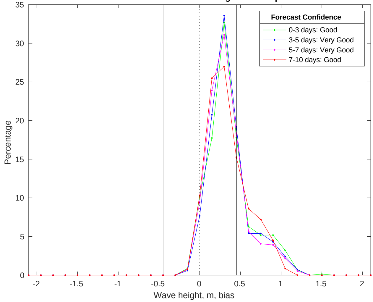
NDBC 51211 vs CMEMS Waves Bias Histogram: 17-Sep-2025
