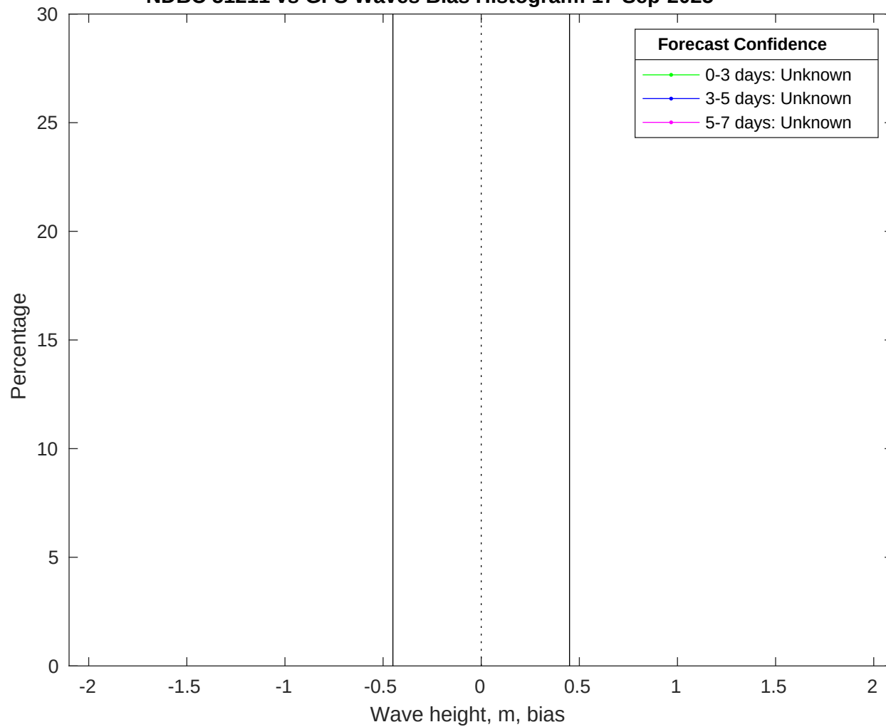
NDBC 51211 vs GFS Waves Bias Histogram: 17-Sep-2025
