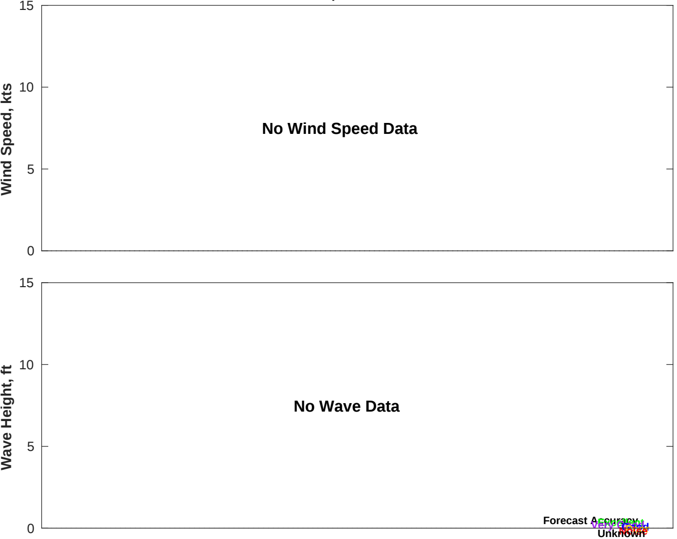
Wind & Wave Forecast for NDBC 51211 from 16-Sep-2025 14:00:00 to 02-Oct-2025 14:00:00
