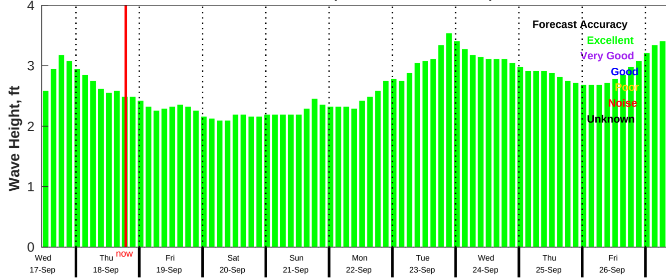
CMEMS Wave Forecast for NDBC 52211 from 16-Sep-2025 11:00:00 to 26-Sep-2025 11:00:00
