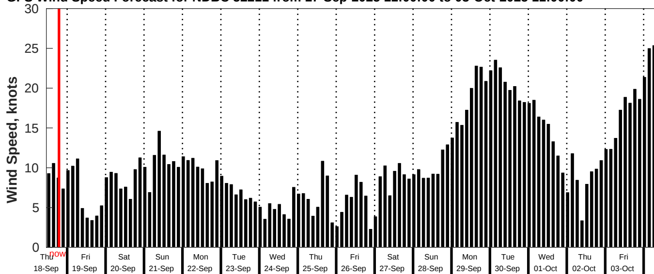
GFS Wind Speed Forecast for NDBC 52211 from 17-Sep-2025 11:00:00 to 03-Oct-2025 11:00:00
