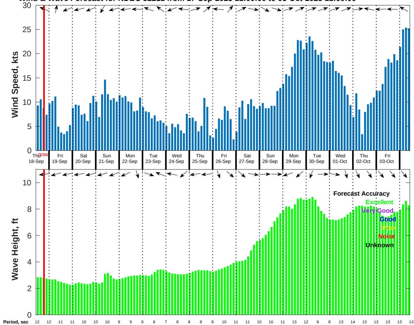
Wind & Wave Forecast for NDBC 52211 from 17-Sep-2025 11:00:00 to 03-Oct-2025 11:00:00
