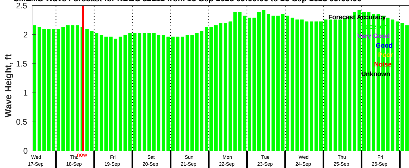
CMEMS Wave Forecast for NDBC 52212 from 16-Sep-2025 09:00:00 to 26-Sep-2025 09:00:00
