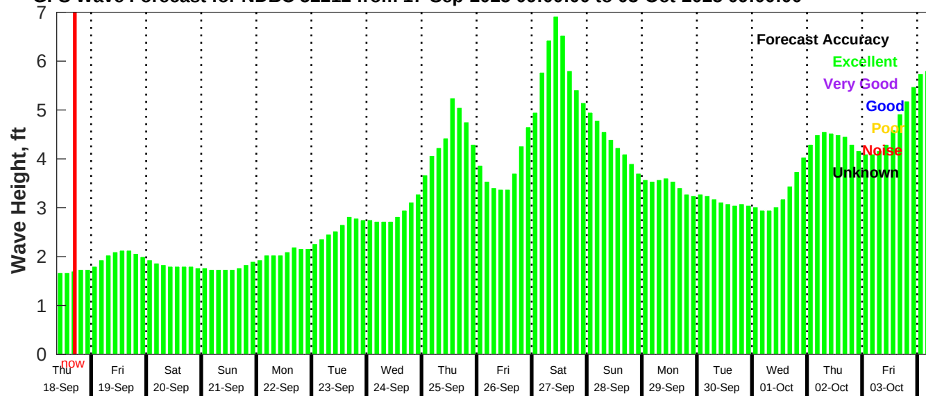
GFS Wave Forecast for NDBC 52212 from 17-Sep-2025 09:00:00 to 03-Oct-2025 09:00:00
