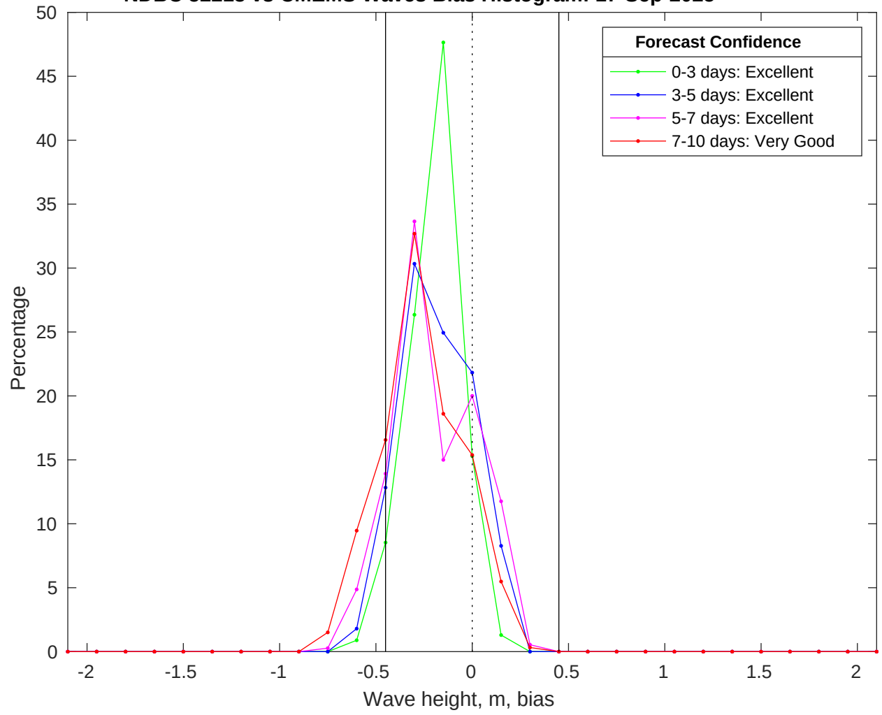
NDBC 52213 vs CMEMS Waves Bias Histogram: 17-Sep-2025
