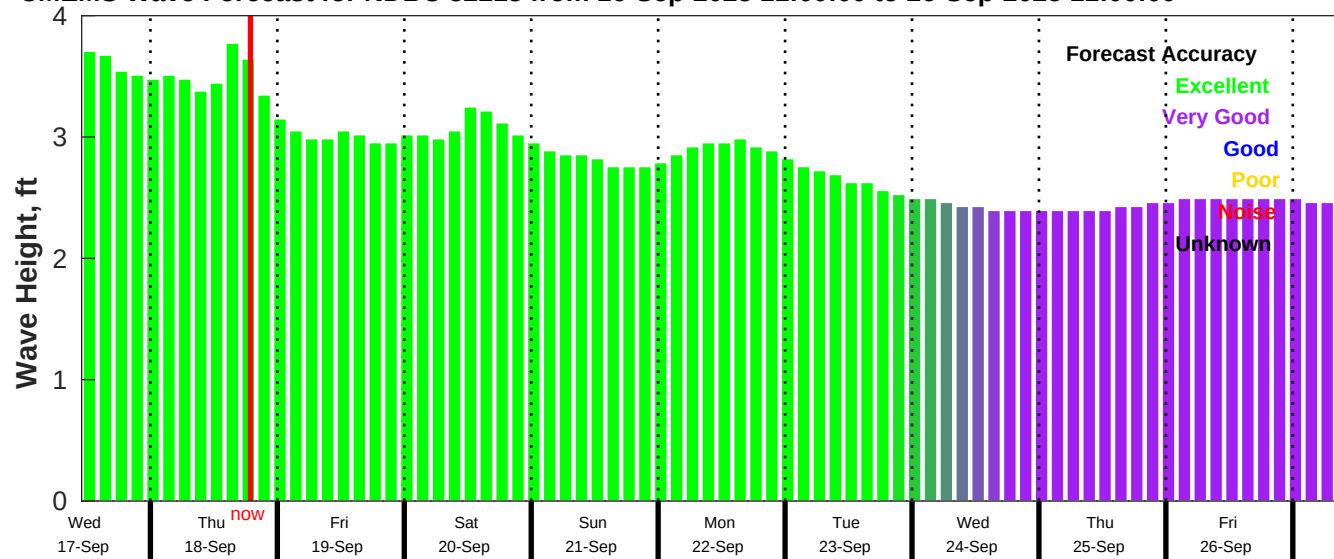
CMEMS Wave Forecast for NDBC 52213 from 16-Sep-2025 11:00:00 to 26-Sep-2025 11:00:00
