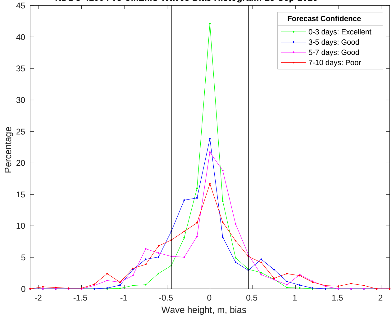
NDBC 41004 vs CMEMS Waves Bias Histogram: 18-Sep-2025
