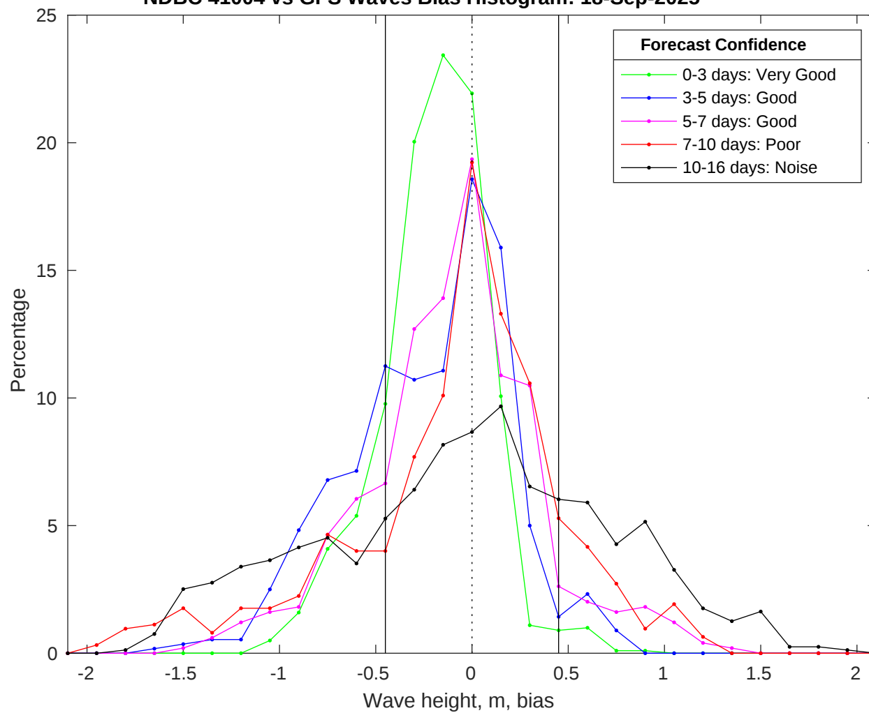
NDBC 41004 vs GFS Waves Bias Histogram: 18-Sep-2025
