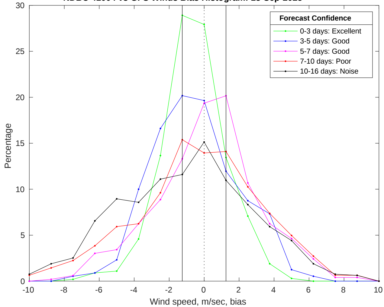
NDBC 41004 vs GFS Winds Bias Histogram: 18-Sep-2025
