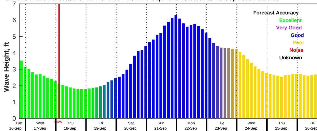
CMEMS Wave Forecast for NDBC 41004 from 16-Sep-2025 19:00:00 to 26-Sep-2025 19:00:00
