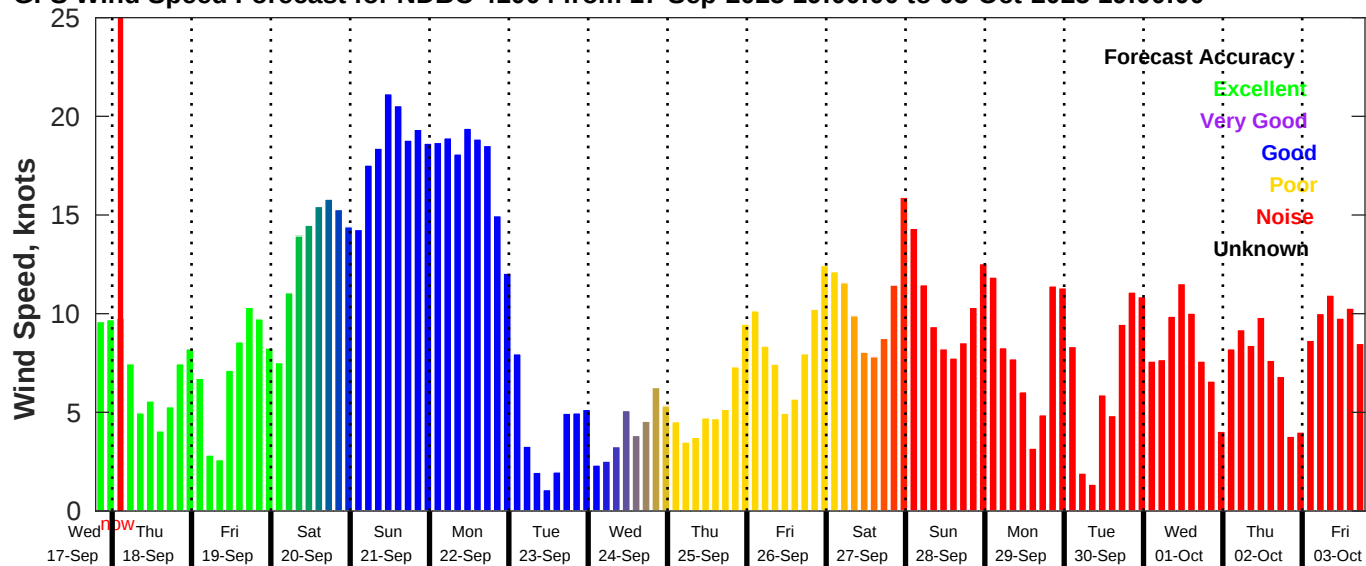
GFS Wind Speed Forecast for NDBC 41004 from 17-Sep-2025 19:00:00 to 03-Oct-2025 19:00:00
