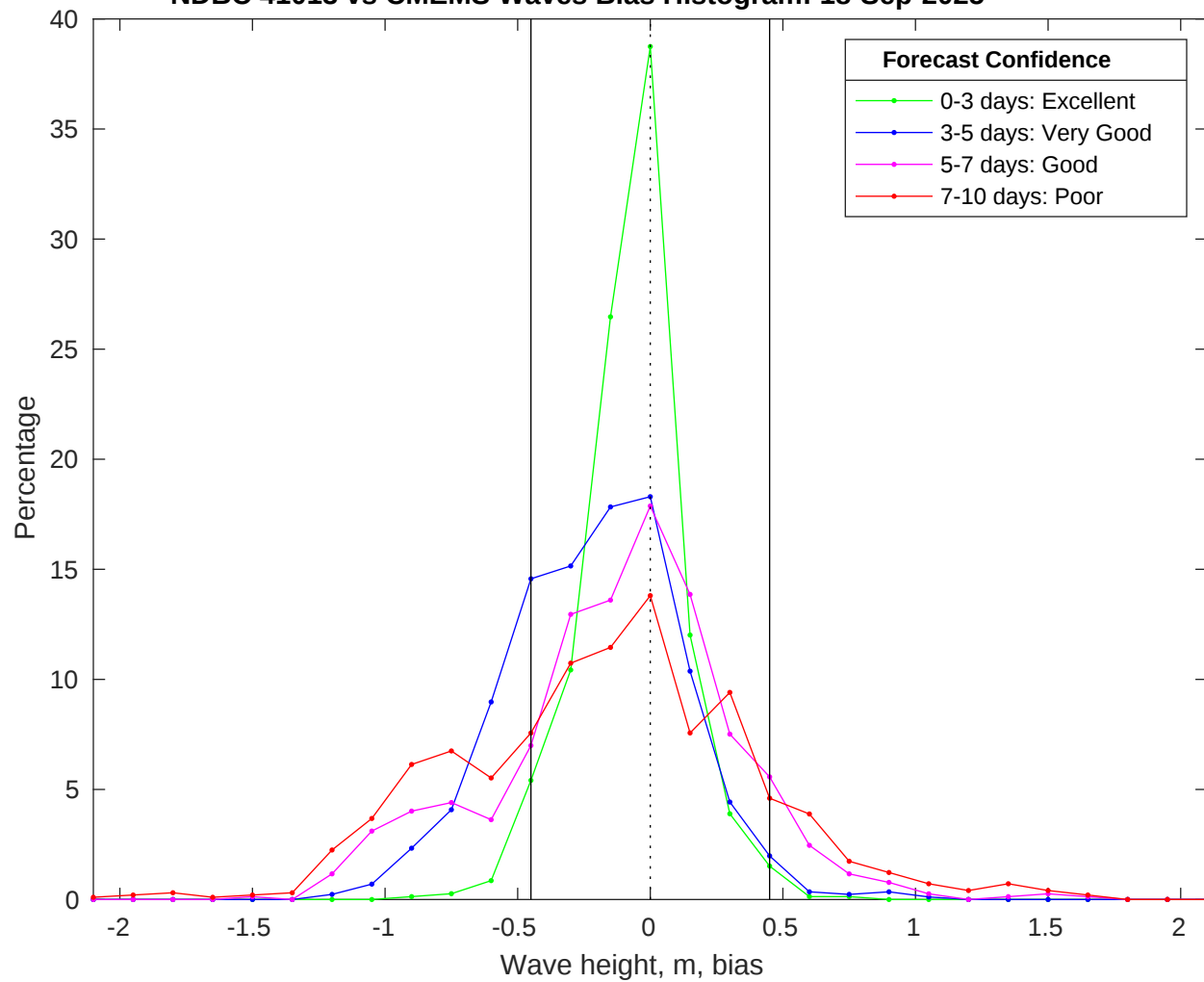
NDBC 41013 vs CMEMS Waves Bias Histogram: 18-Sep-2025
