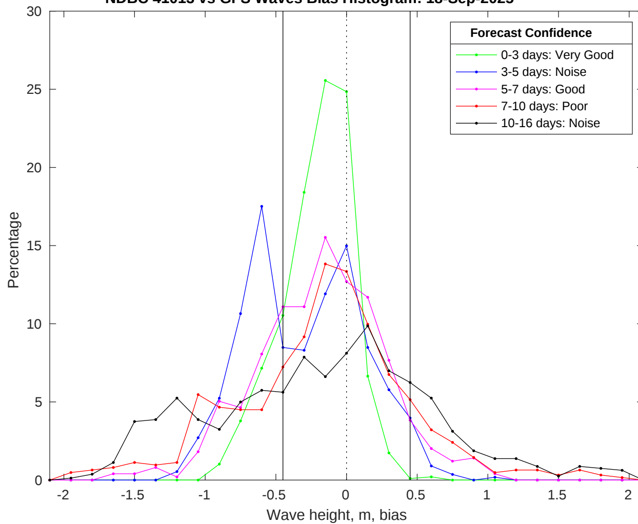
NDBC 41013 vs GFS Waves Bias Histogram: 18-Sep-2025
