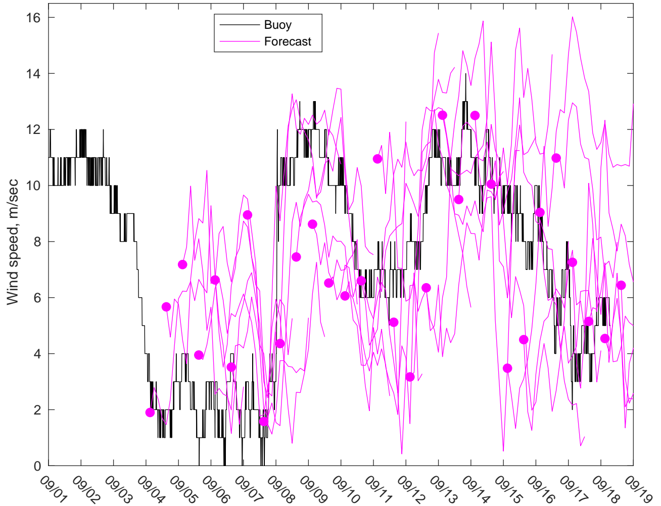
NDBC 41013 vs GFS Winds: 7 to 10 day forecast
