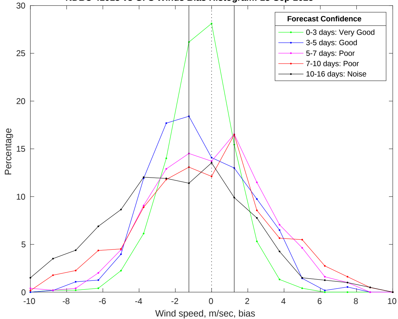
NDBC 41013 vs GFS Winds Bias Histogram: 18-Sep-2025
