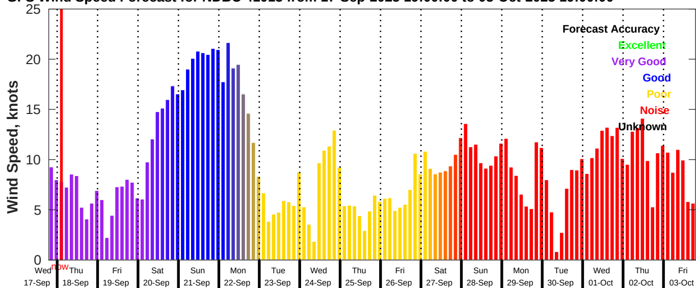
GFS Wind Speed Forecast for NDBC 41013 from 17-Sep-2025 19:00:00 to 03-Oct-2025 19:00:00
