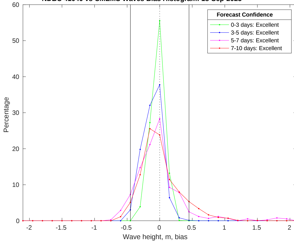
NDBC 41040 vs CMEMS Waves Bias Histogram: 18-Sep-2025
