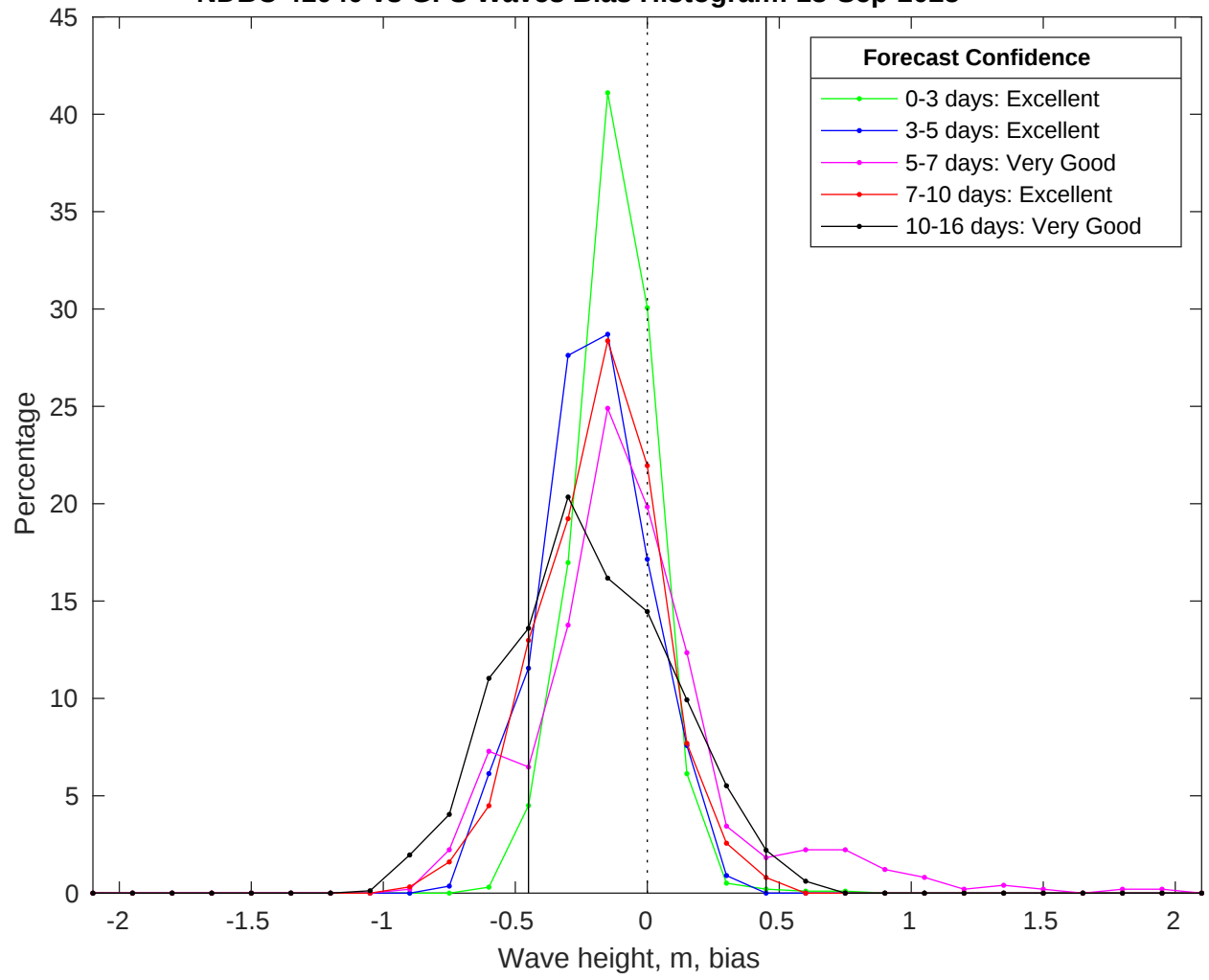
NDBC 41040 vs GFS Waves Bias Histogram: 18-Sep-2025
