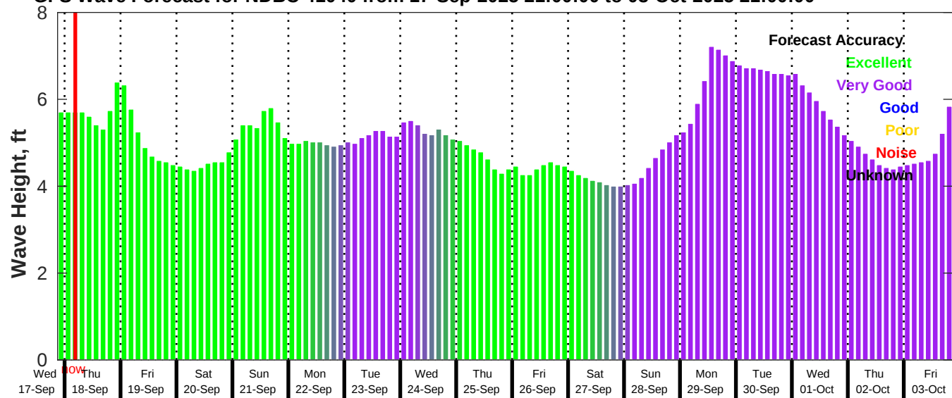
GFS Wave Forecast for NDBC 41040 from 17-Sep-2025 21:00:00 to 03-Oct-2025 21:00:00
