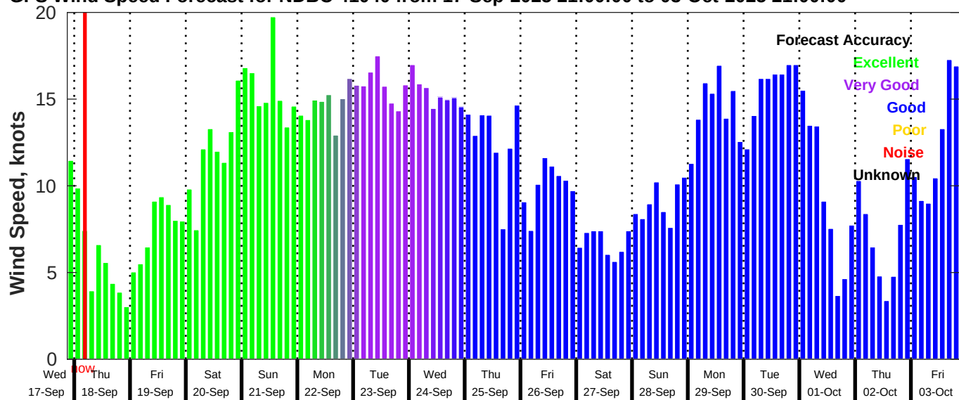
GFS Wind Speed Forecast for NDBC 41040 from 17-Sep-2025 21:00:00 to 03-Oct-2025 21:00:00
