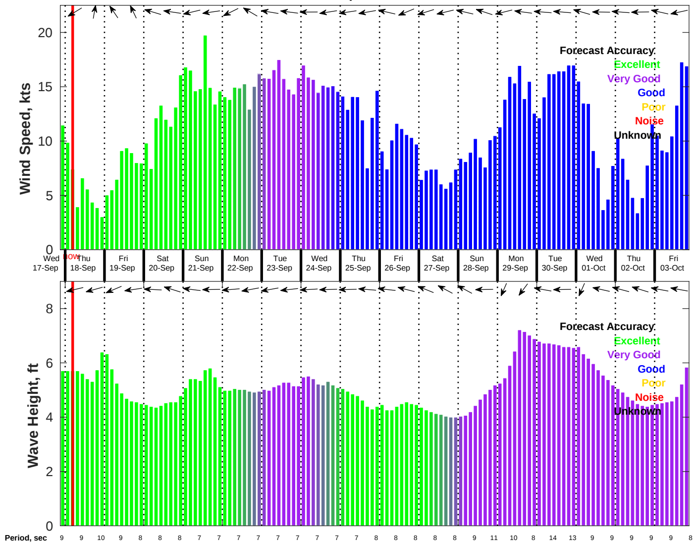
Wind & Wave Forecast for NDBC 41040 from 17-Sep-2025 21:00:00 to 03-Oct-2025 21:00:00
