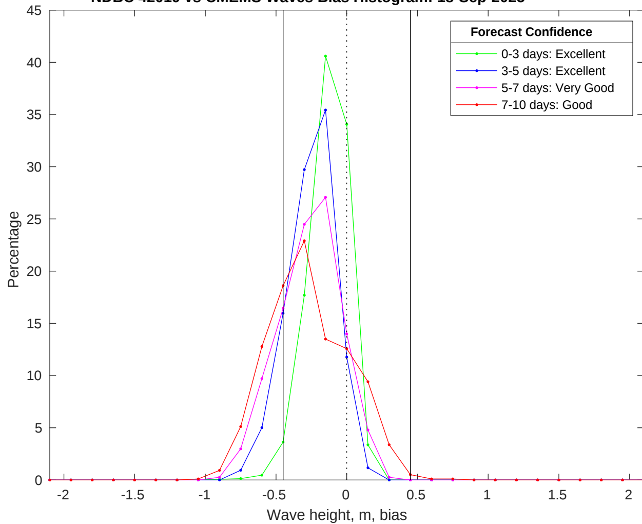
NDBC 42019 vs CMEMS Waves Bias Histogram: 18-Sep-2025
